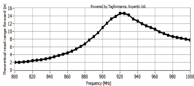
读距范围 (m) Read Range
