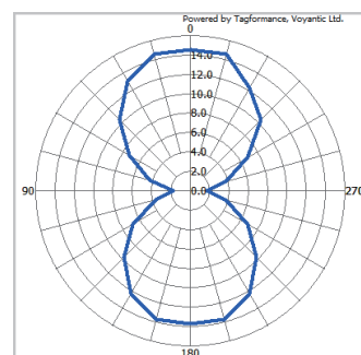
方位性 Orientation Sensitivity
